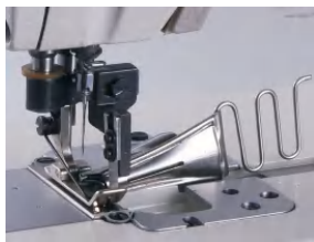
切包一体 Cutting and binding
