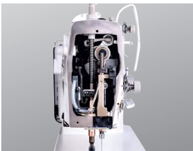
高精度针杆架 High accuracy needle bar frame
